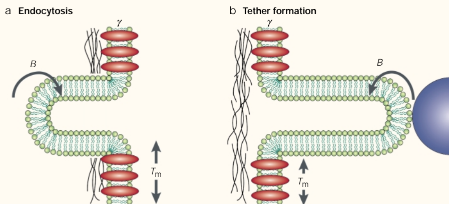
Figure 1 | The energetics of endocytic vesicle formation are similar to those of tether formation. This diagram illustrates that the factors that contribute to the load of forming a vesicle are the same as those that contribute to forming a tether. The major factor is the membrane–cytoskeleton adhesion energy, \gamma , which must be overcome to separate membrane from cytoskeleton. A secondary term is the tension in the bilayer plane, T_m , which resists deformation of the membrane. Because the curvature of vesicles and tethers are similar, the force needed to bend the membrane should be similar (membrane bending stiffness, B , defines the force for a given radius of curvature 39 ). See Box 1 for details.
