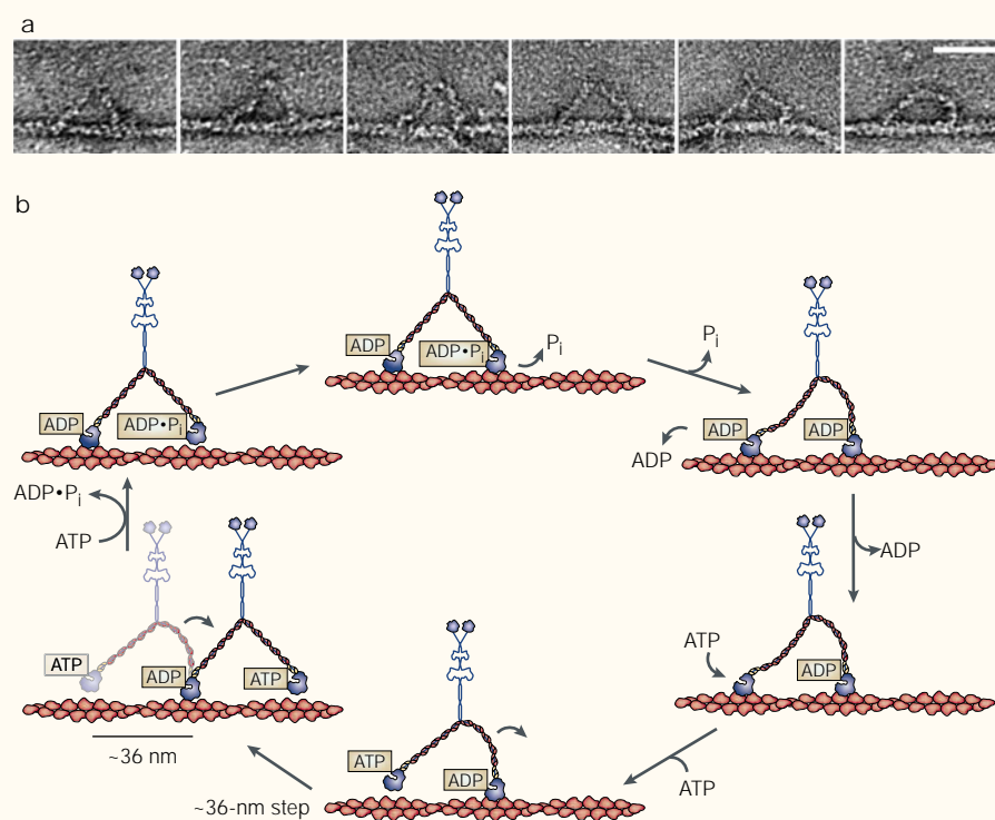
Figure 6 | Nucleotide-dependent processive stepping of myosin V along an actin filament. a | The electron micrograph images reveal the two heads of myosin V bound to the actin filament with a separation of \sim 30 nm, or straddling 11 actin monomers, in the three panels on the left. The three panels on the right show binding of the two heads with a separation of \sim 36 nm, or straddling 13 actin monomers. Some images show a configuration reminiscent of a 'telemark skier.' Bar, 36 nm. Adapted with permission from REF. 39 © (2000) Macmillan Magazines Ltd. b | A model for myosin-V stepping. As illustrated in the lower right panel, myosin V dwells with both heads attached to the actin filament, the leading head with ADP and the trailing head in rigor. ATP binding to the trailing head promotes its dissociation from actin, and forward movement of the released head then discharges intramolecular strain. The previous leading head then becomes the trailing head (lower left panel). Note that the trailing head moves 72 nm to reach its new site of attachment, but this results in only a 36-nm step of the body of myosin V or of any cargo attached to the cargo attachment domain. The new, detached leading head quickly hydrolyses ATP and then binds actin. Force generation follows either actin binding or phosphate release, which itself occurs either concomitant with or immediately following actin binding. These steps are fast relative to ADP release. At this point, the molecule is in its kinetically dominant state: both heads bound to actin and ADP, the leading head in a prestroke configuration and the trailing head in a poststroke configuration (upper right). The leading head is stressed against the direction of motion and the trailing head is stressed along this direction, an asymmetry that should bias the following ADP release to occur at the trailing head and not the leading head.
