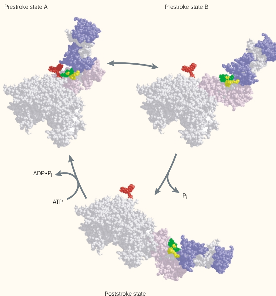
Figure 2 | Prestroke and poststroke states of subfragment 1. Structures modelled from the prestroke and poststroke subfragment 1 (S1) crystal structures 18–21 are shown, with the catalytic domain of S1 kept in a fixed orientation. The lever arm moves through an angle of ~70°, going from prestroke state A to the poststroke state. Prestroke state B was predicted from fluorescence resonance energy transfer (FRET) measurements 28 . The red colour shows the position of an acceptor dye for the FRET measurements. The green and yellow colours show two independent positions for placing a donor dye on the regulatory light chain. Adapted from REF. 28. © (2000), with permission from Elsevier Science.
