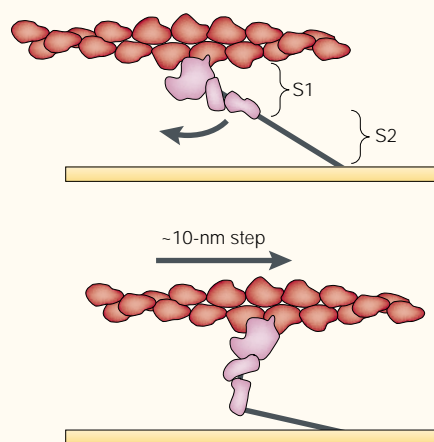
Figure 1 | The swinging cross-bridge model. The model shown is that of H.E. Huxley 1 , modified to indicate bending near the middle of the elongated cross-bridge (subfragment 1, or S1) to provide the working stroke. The S1 is tethered to the bipolar thick filament (horizontal yellow line) through the S2 domain of the myosin molecule. The actin filament structure is based on the model proposed by Holmes et al. 44 , and the S1 structures are based on various crystal structures 18–21 . S1 and filamentous actin (F-actin) are drawn to scale.
