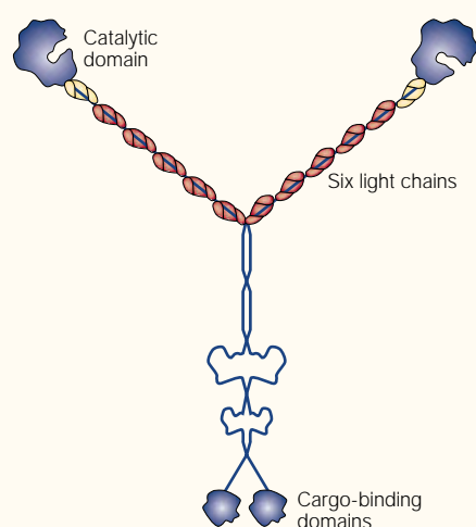
Figure 4 | Predicted structure of myosin V. The putative lever arm of myosin V is roughly threefold longer than that of myosin II. The tail domain is also different between the two myosin types because the tail of myosin V functions to bind vesicular cargo in non-muscle cells as opposed to myosin II, which functions to form bipolar thick filaments for contractile events.
