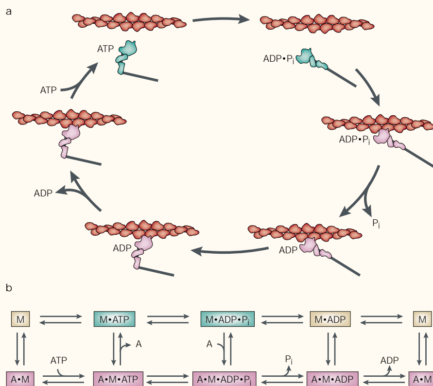
Figure 3 | The actin-activated myosin-II ATPase cycle. a | The states of the myosin subfragment 1 (S1) domain that are strongly attached to actin are shown in pink. Myosin II is only strongly attached ~5% of the total time of the cycle. That is, the myosin spends most of its time off the actin or only weakly associated (green states). The structures shown were modelled as described in FIG. 1. b | All of the myosin and actin–myosin nucleotide states are shown. All steps are reversible. A, actin; M, myosin. A primary path corresponding to the structures shown in a is A•M to AM•ATP to M•ATP to M•ADP•P i to AM•ADP•P i to AM•ADP to AM.
